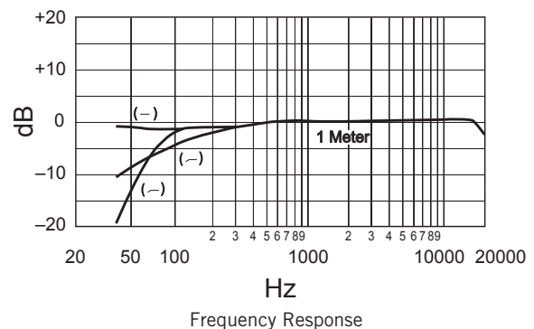
Frequency Response
